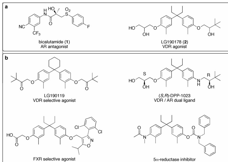
Figure 1. (a) Chemical structures of representative non-steroidal NR ligands. (b) Diphenylpentane-based ligands of NR and steroid-related enzyme generated by means of the multi-template approach.
