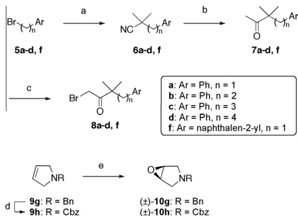
Scheme 1. Reagents and conditions: (a) LDA, isobutyronitrile, THF, 0 °C to rt, 67–97%; (b) MeLi, THF, 0 °C to rt, 35–94%; (c) Br 2 , 1,4-dioxane, 0 °C to rt, quant.; (d) CbzCl, KHCO 3 , CHCl 3 , rt, 48%; (e) mCPBA, H 2 SO 4 , acetone, H 2 O, rt, 12–40%.
