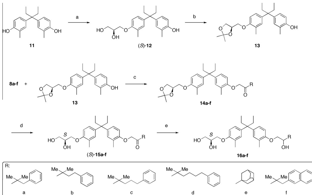
Scheme 2. Reagents and conditions: (a) (S)-glycidol, CsF, DMF, 85 °C, 47%; (b) acetone dimethyl acetal, CSA, MeCN, rt, 87%; (c) K 2 CO 3 , DMF, rt or 90 °C, 21–71%; (d) TsOH, MeOH, THF, rt, 30–69%; (e) NaBH 4 , MeOH, rt, 37–83%.
