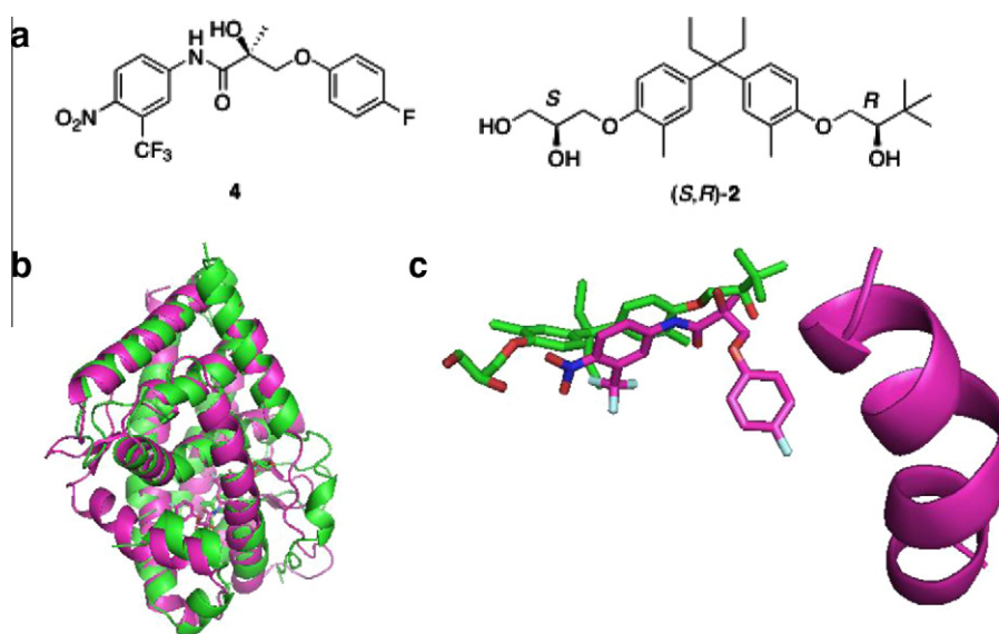
Figure 2. (a) Chemical structures of bicalutamide analog 4 and ( S,R )- 2 . (b) Superposition of X-ray crystal structures of the complex of AR with 4 (magenta, PDB ID: 2AXA) and the complex of VDR with ( S,R )- 2 (green, PDB ID: 2ZFX). (c) Overlay of active conformation of ( S,R )- 2 (green stick) and 4 (magenta stick), and helix 12 of AR (magenta ribbon). The images were drawn with PYMOL.
