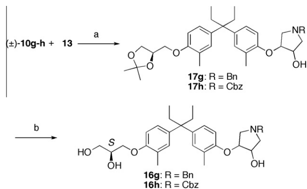
Scheme 3. Reagents and conditions: (a) Cs 2 CO 3 , 18-crown-6, EtOH, reflux, 22–29%; (b) TsOH, MeOH, THF, rt, 78–80%.
